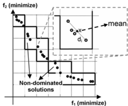
Figure 5. Clustering scheme [22].
